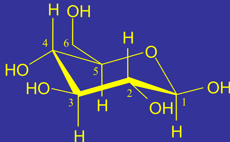
\beta -D-glucopyranose
