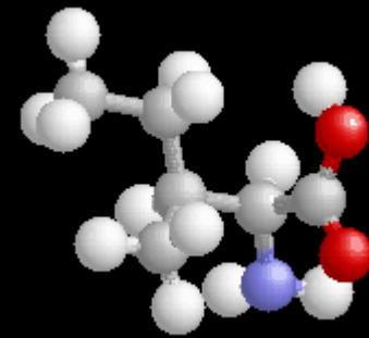
Isoleucine
