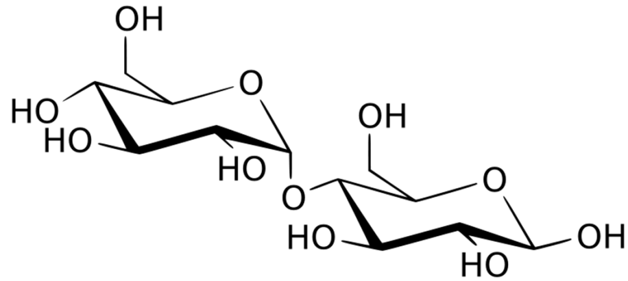
Maltose
