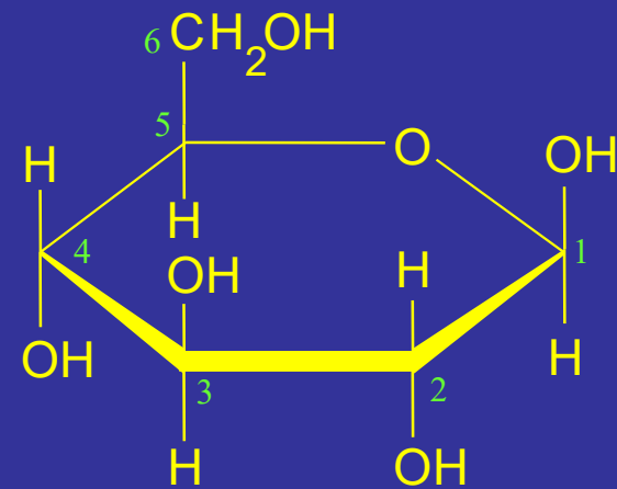
\beta -D-glucose
