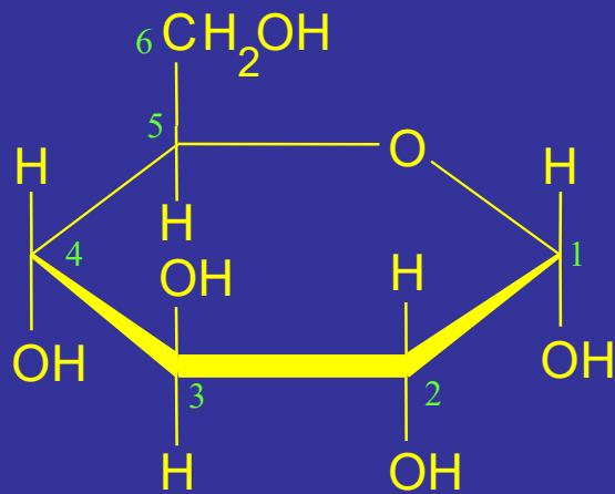
\alpha -D-glucose
