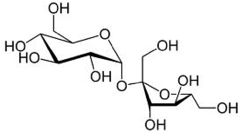
Sucrose
